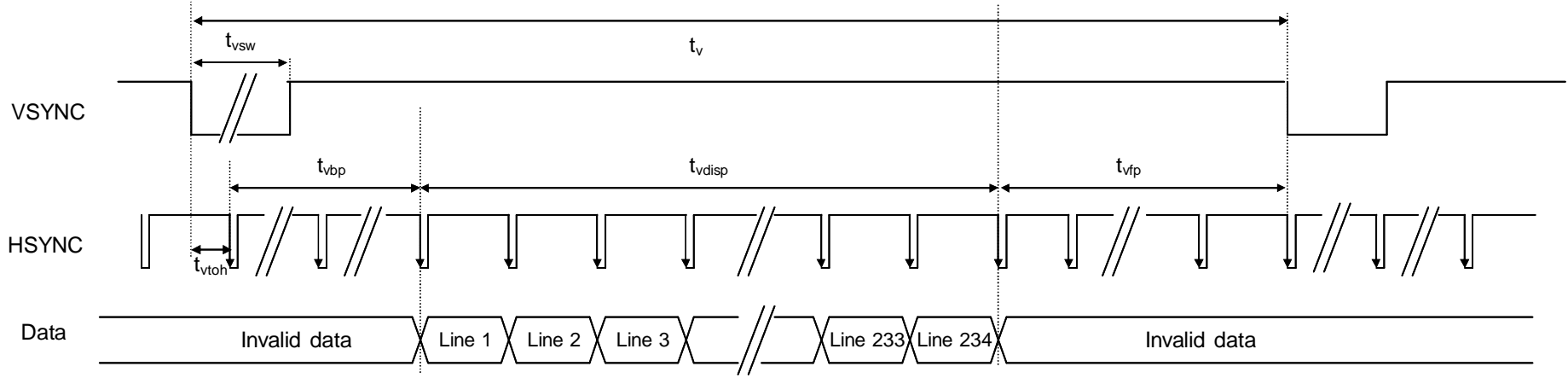
Even Field
