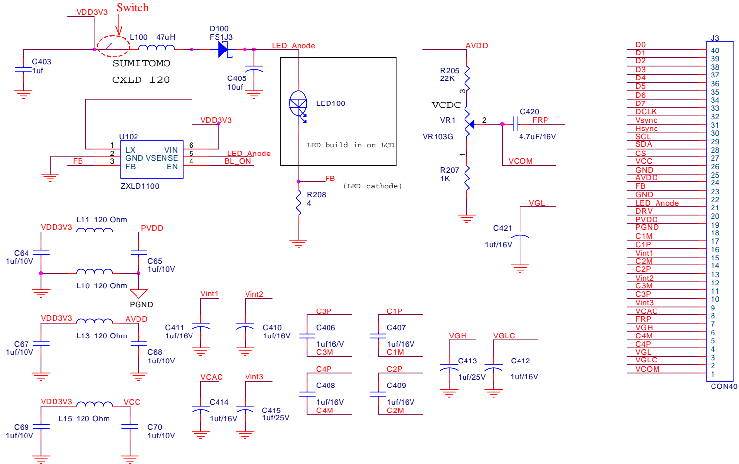
External AVDD + External LED Driver Application Circuit
