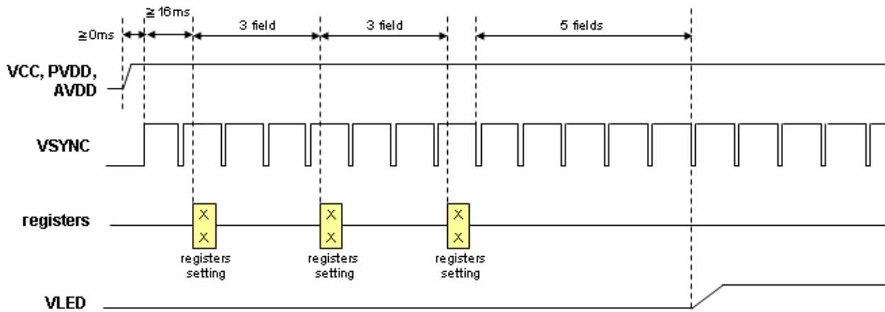
Fig. 3 LCD serial command setting during power on
