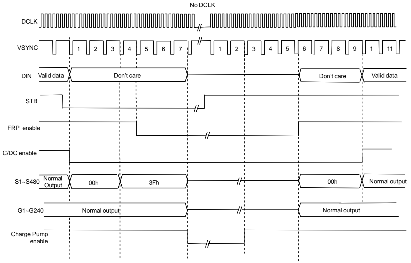
Fig. 2 Stand-by timing diagram
